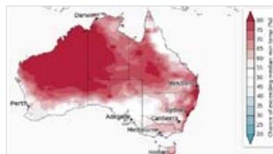
Temperature - Chance of above median minimum temperature for August to October.
