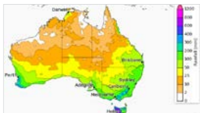
Rainfall - Totals that have a 50% chance of occurring for August to October
